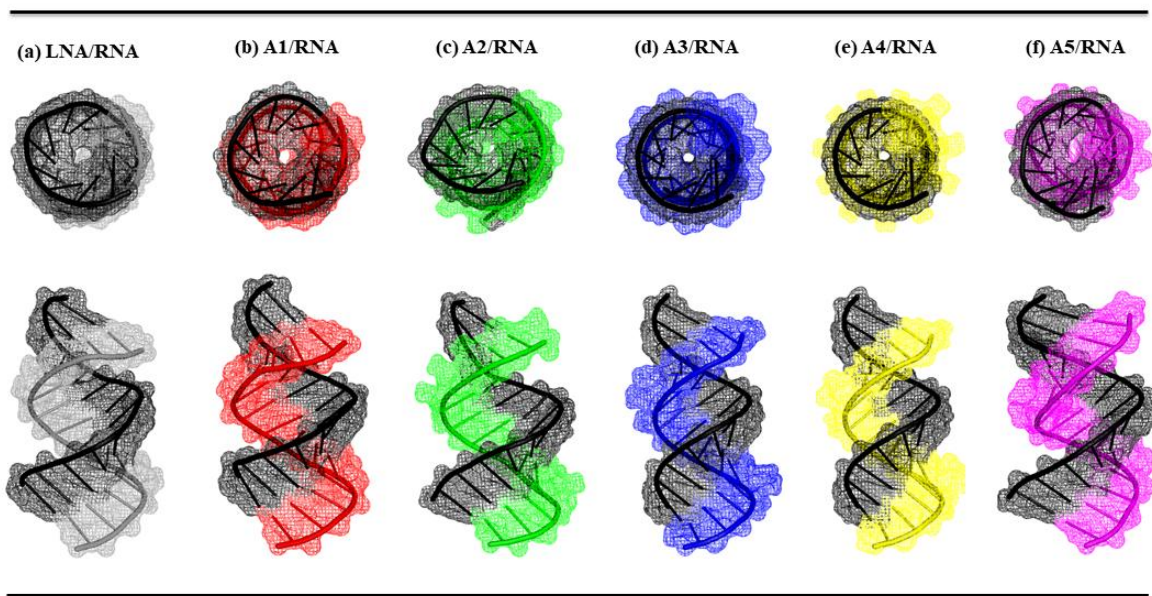
14-mer (5'-CTTAGCACTGGCCT-3'/5'-AGGCCAGUGC UAAG-3') ASO/RNA duplexes
