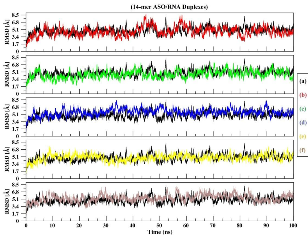
Figure 6: RMSD plots of the 14-mer ASO/RNA duplexes (a) LNA/RNA (b) A1/RNA (c) A2/RNA (d) A3/RNA (e) A4/RNA and (f) A5/RNA for the entire simulation trajectory.
