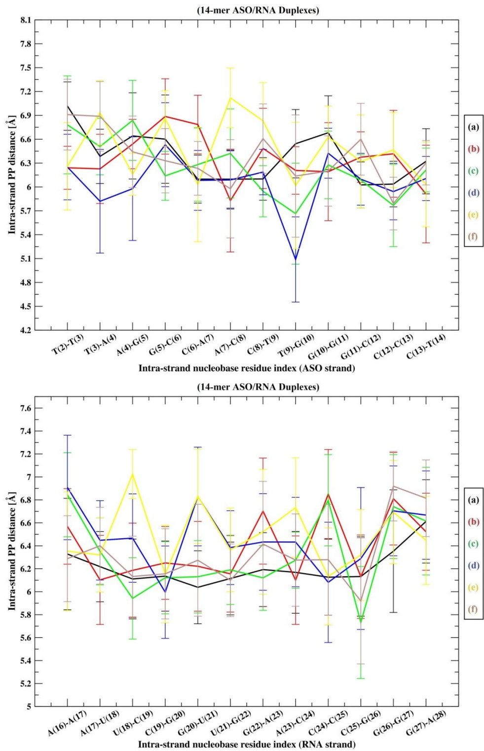
Figure 7: Inter-strand and Intra-strand PP distances of the 14-mer ASO/RNA duplexes (a) LNA/RNA (b) A1/RNA (c) A2/RNA (d) A3/RNA (e) A4/RNA and (f) A5/RNA for both the strands for the entire simulation trajectory.
