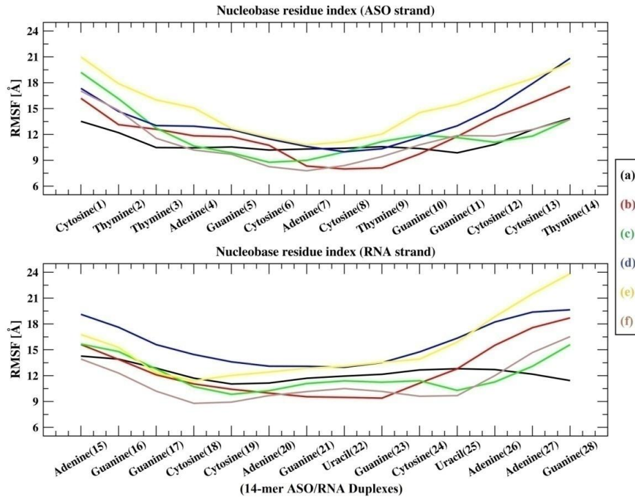
Figure 10: Backbone flexibility of monomer nucleotides of the 14-mer ASO/RNA duplexes (a) LNA/RNA (b) A1/RNA (c) A2/RNA (d) A3/RNA (e) A4/RNA and (f) A5/RNA for both the antisense and the sense strand for the entire simulation trajectory.
