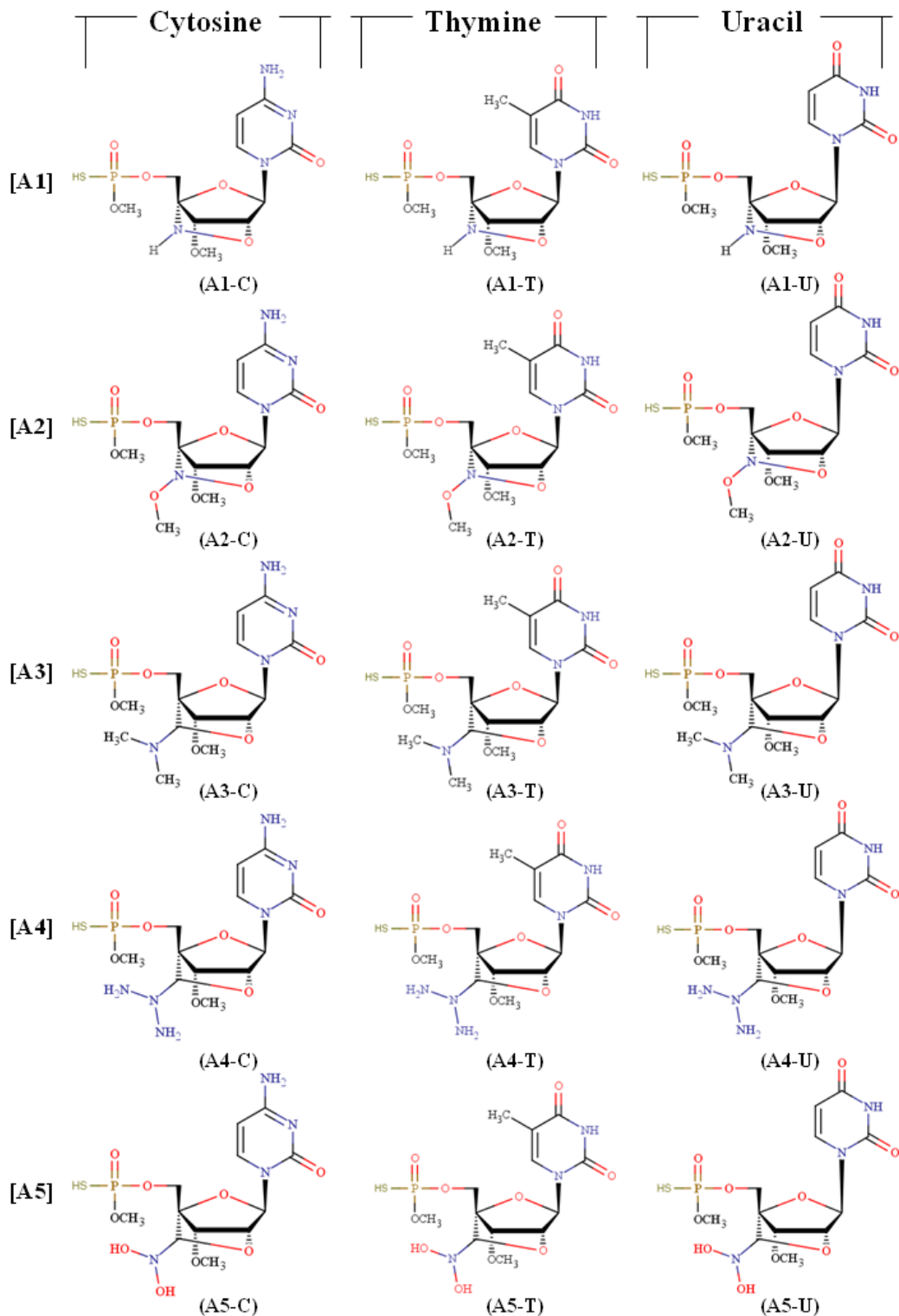
Figure 1: Schematic 2D representation of the proposed LNA analogue antisense modifications A1, A2, A3, A4, A5 each containing nucleobases Adenine(A), Guanine(G), Cytosine(C), Thymine(T) and Uracil(U), respectively.
