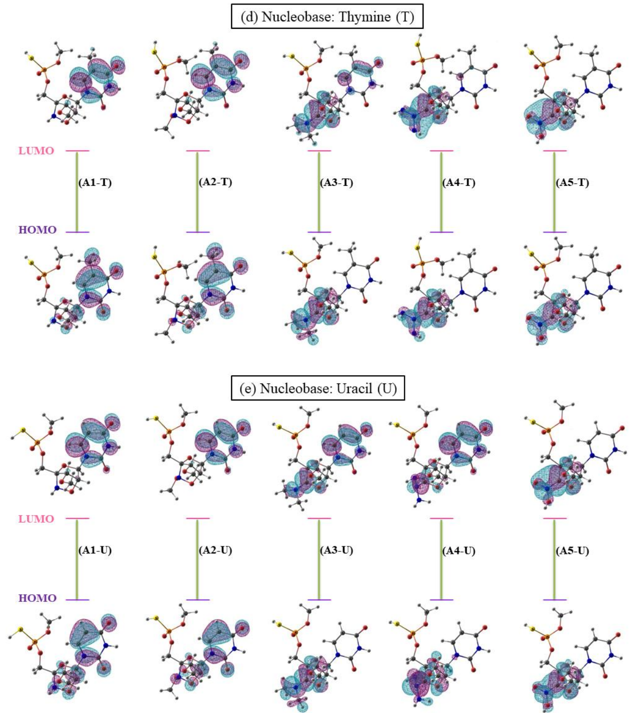
Figure 4: HOMO, LUMO iso-surfaces of monomer nucleotides of the proposed LNA analogue antisense modifications (A1-A5) each containing nucleobase (a) Adenine(A), (b) Guanine(G), (c) Cytosine(C), (d) Thymine (T) and (e) Uracil (U) respectively calculated at the M06-2X/6-311G(d,p) level of theory.
